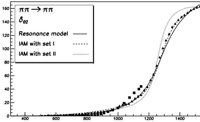
FIG. 1. Experimental data ([12] squares, [13] circles, [14] triangles) on the I = 0, J = 2 \pi\pi scattering phase shift and the results of our unitarized chiral resonance model (continuous line), of eq.(8) with the parameters in set I (dashed line), and with those in set II (dotted line)
